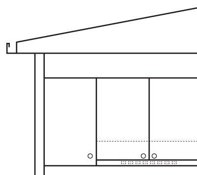
FRONT RE-CIRCULATING (Carbon filter required)
